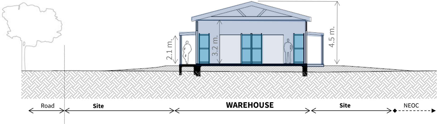
Section B
