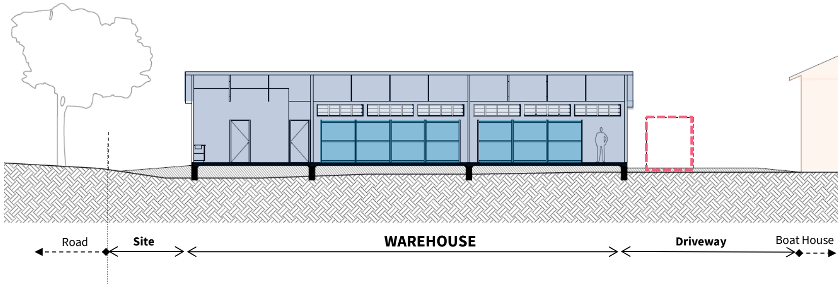
Section B
